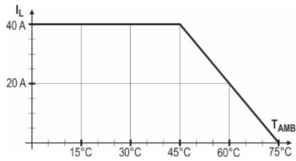
Figura 3 – SSR4840 + dissipador ND40-100 mm
